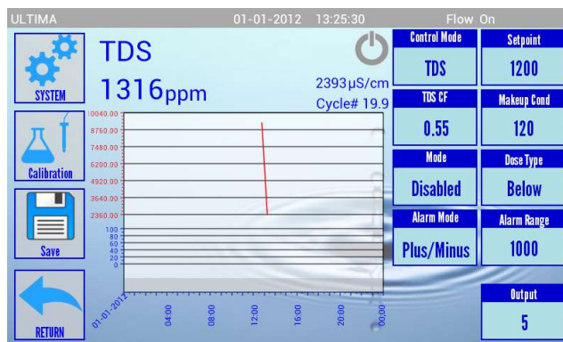
Picture 15 TDS/CONDUCTIVITY Screen
