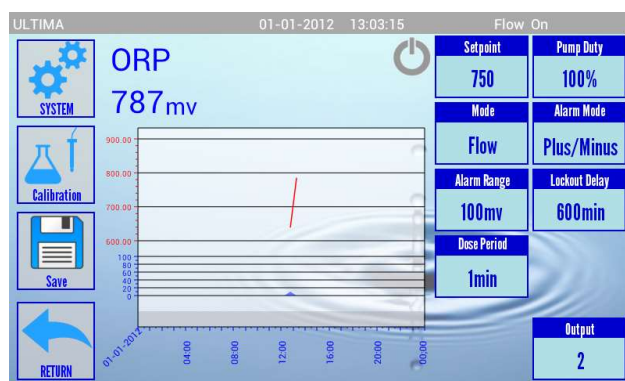
Picture 13. ORP screen
