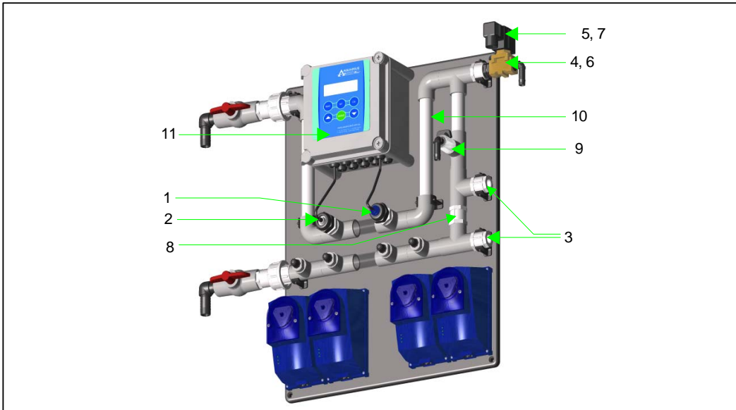
Tower controller, ORP, pH, conductivity
